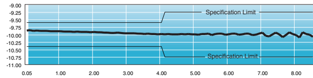
Typical Attenuation Accuracy of a 24-10-34
