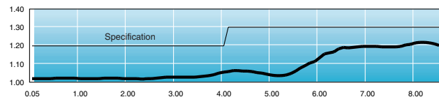
Typical SWR of a 24-10-34
