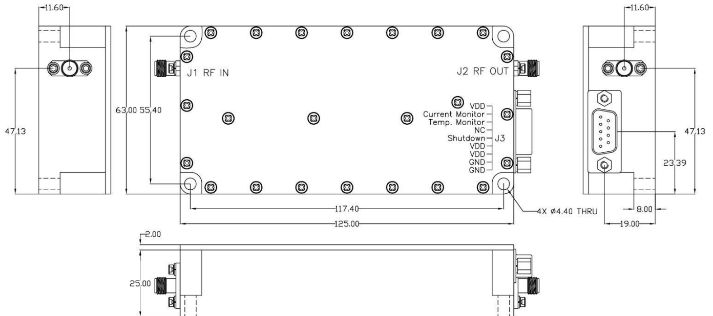
OUTLINE DRAWING – SHOWN WITH OPTION 101
