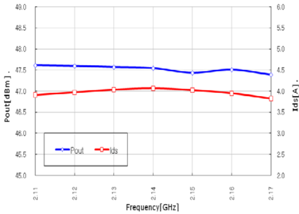
Output Power @ Pin=14dBm & Ids vs. Frequency
