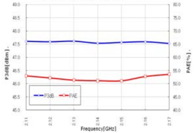
P3dB & PAE vs. Frequency
