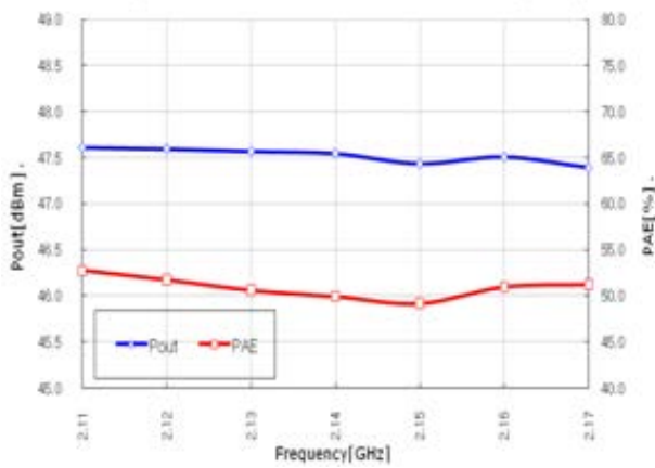
Output Power @ Pin=14dBm & PAE vs. Frequency
