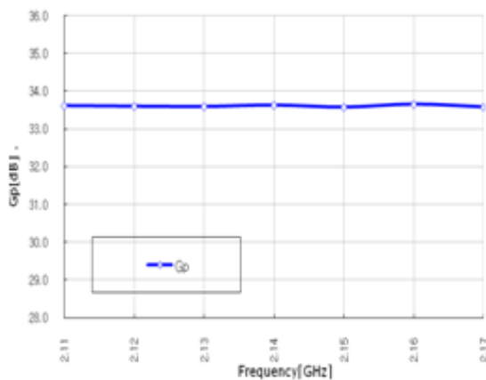
Power Gain @ Pin=14dBm vs. Frequency
