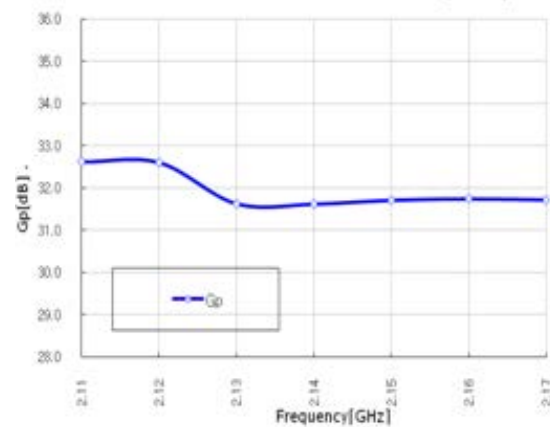
Power Gain @ P3dB vs. Frequency
