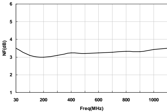
Noise Figure
