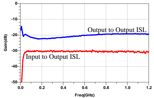
Isolation
