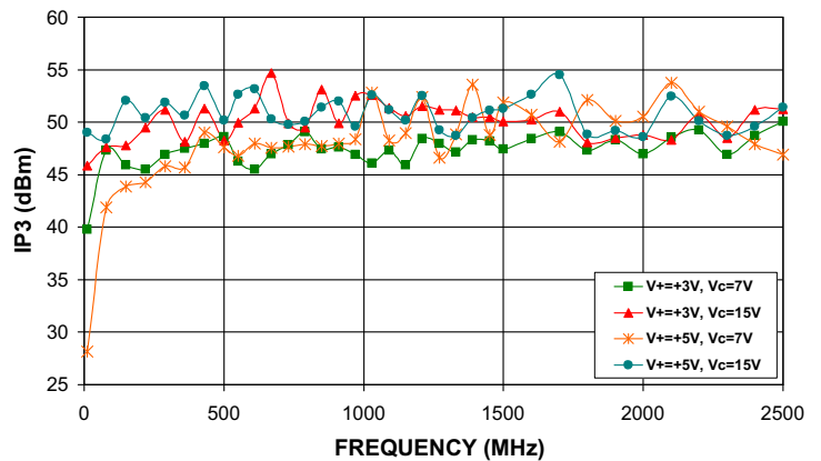
RVA-2500-75+ IP3 Vs. FREQUENCY
