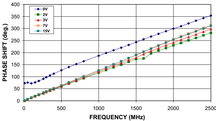
RVA-2500-75+ PHASE SHIFT Vs. FREQUENCY OVER CONTROL VOLTAGES @ V+=3V
