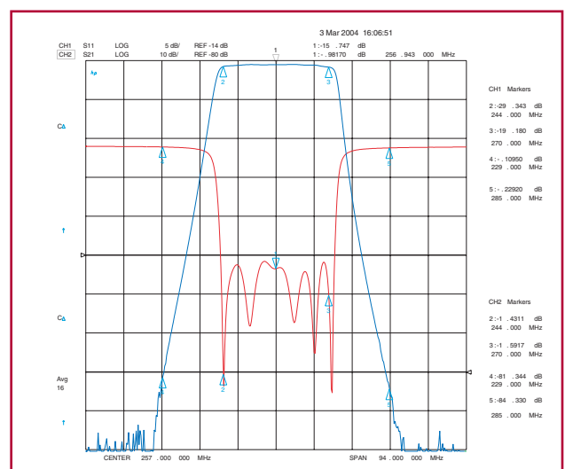
Passband & Return Loss
