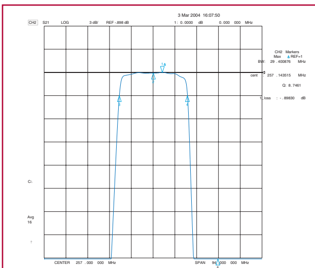
3 dB BW
